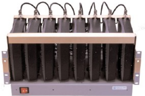
SX5 Multi-Line 19" Rack System, for permanent installation Supports up to 8 SX5 line modules, shares single antenna
