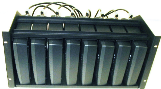
CT-8 Multi-Line 19" Rack System, for permanent installation Supports up to 8 SX5 line modules, shares single antenna
